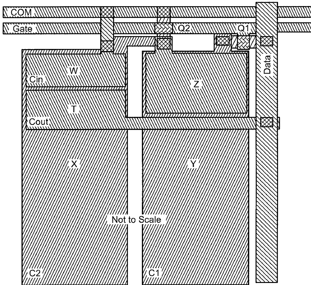
Subpixel Layout
